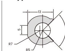
R-Type Rail for \Phi 10
