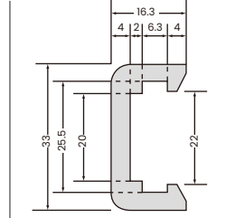
All Type Rail
