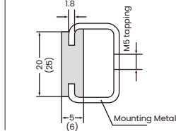
H-Type Rail
