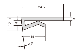
Snap-on Rail
