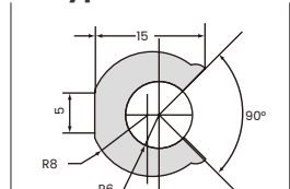
R-Type Rail for \Phi 12
