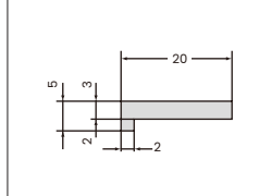
L-Type Rail
