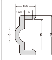
Snap-on Rail
