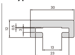
K-Type Rail
