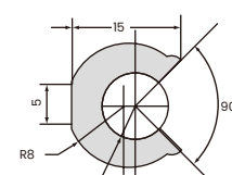
R-Type Rail for \Phi 12
