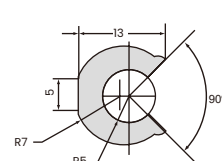
R-Type Rail for \Phi 10
